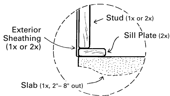
Areas to be treated on a slab.
